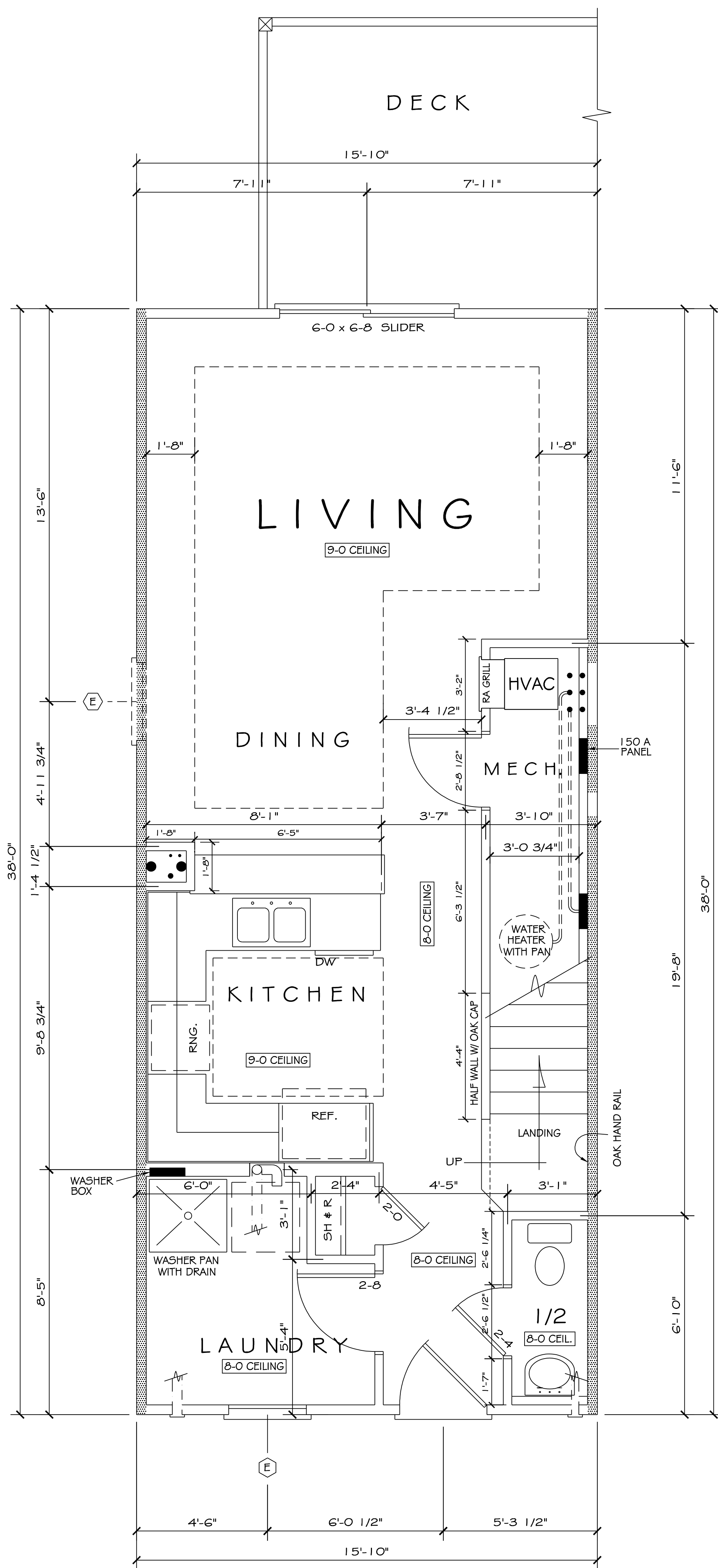
TWO BEDROOM UNIT - MAIN FLOOR
