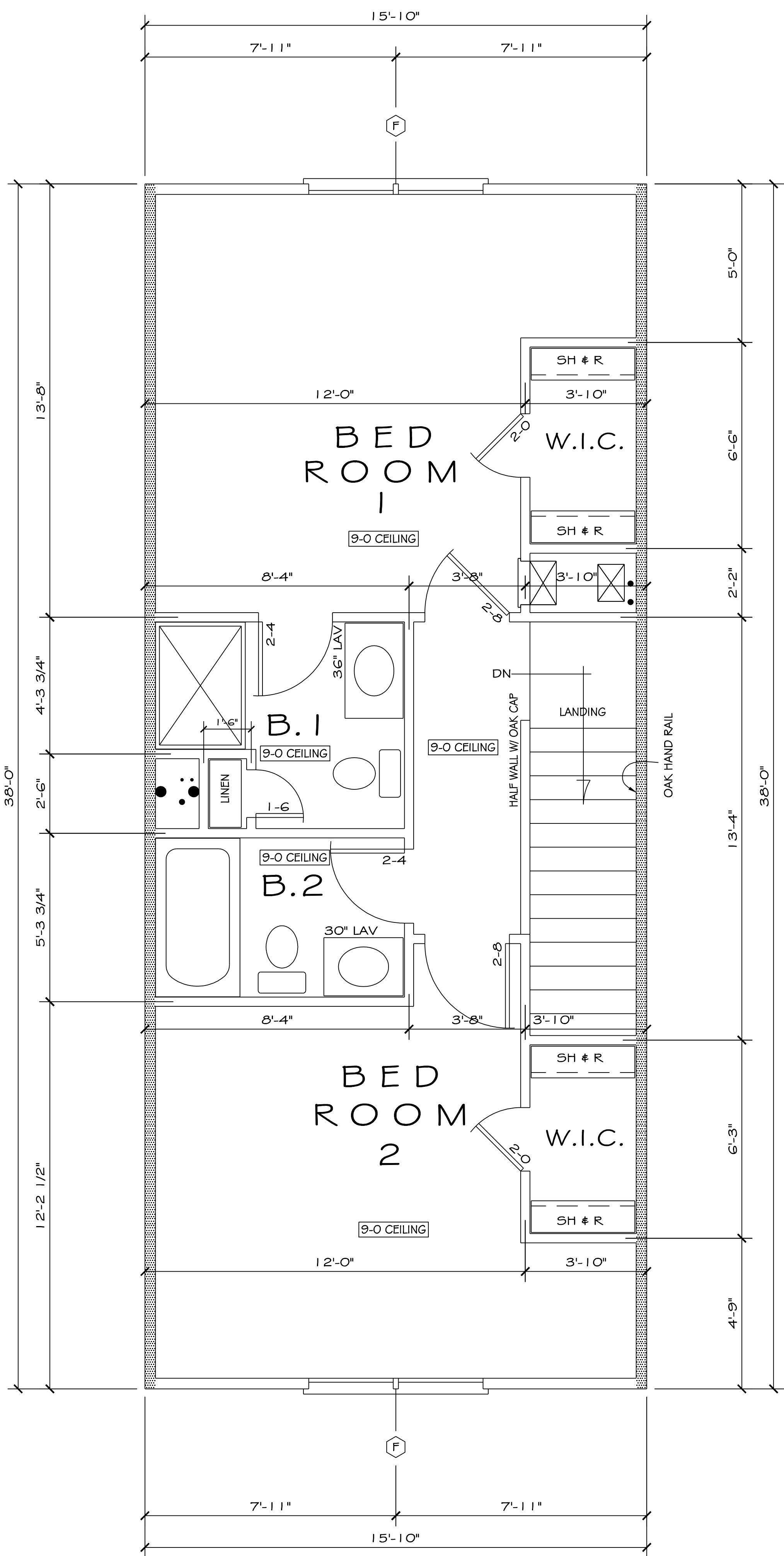
TWO BEDROOM UNIT - UPPER FLOOR
